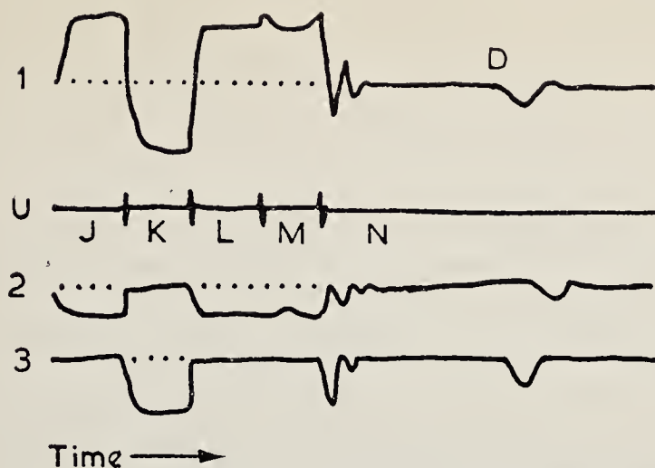
FIGURE 16/8/1: Three units of the Homcostat interacting. Bars in the central positions prevent 2 and 3 from moving in the direction corresponding here to upwards. Vertical strokes on U record changes of unselector position in unit 1. Disturbance D , made by the operator, demonstrates the whole's stability.
