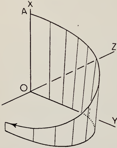
FIGURE 4/5/3: One line of behaviour in the field of the Watt's governor. For clarity, the resting state of the system has been used as origin. The system has been displaced to A and then released.
