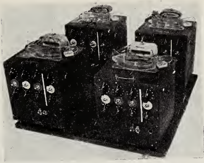
FIGURE 8/2/1 : The Homeostat. Each unit carries on top a magnet and coil such as that shown in Figure 8/2/2. Of the controls on the front panel, those of the upper row control the potentiometers, those of the middle row the commutators, and those of the lower row the switches S of Figure 8/2/3.
